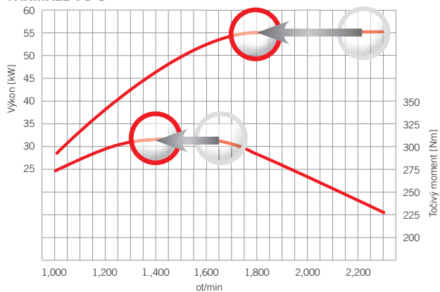
FARMALL 75 C
